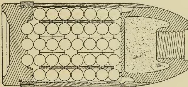
MODERN SHRAPNEL.
